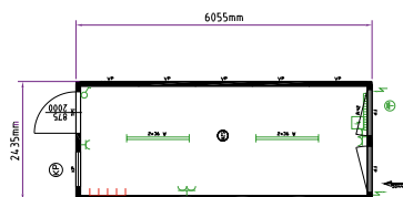
Bungalow bureau 20'
