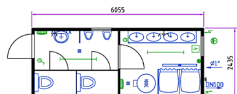
Sanitairunit 20'
