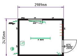
Office cabin 10'
