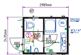
Sanitary cabin 10'
