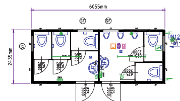
WC cabin ladies/mens 20'
