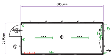
Office cabin 20'
