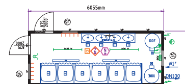
Shower cabin 20'
