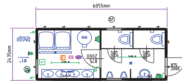
Sanitary cabin 20'
