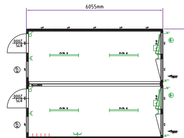
Office cabin double installation
